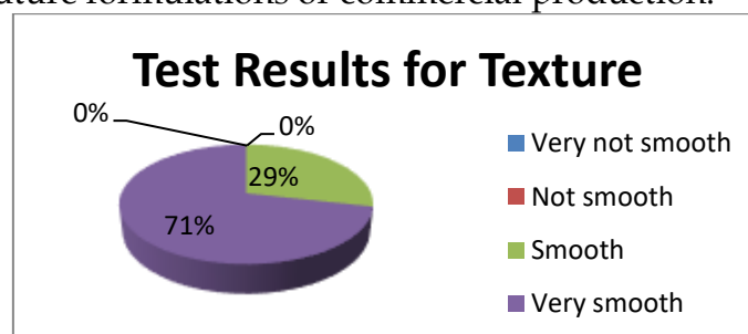
Figure 1. Result of the Texture Organoleptic Test
