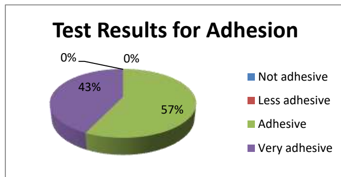
Figure 3. Result of the Adhesion Organoleptic Test
