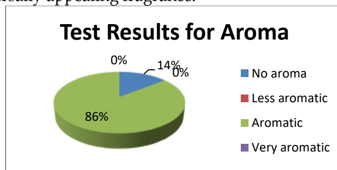
Figure 2. Result of the Aroma Organoleptic Test
