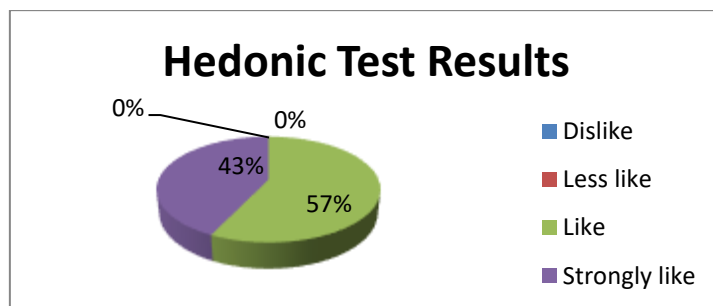
Figure 4. Hedonic Test Result
